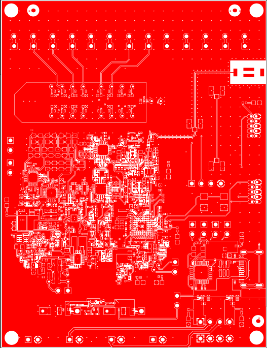
GND 2 (Scale 1:1)
