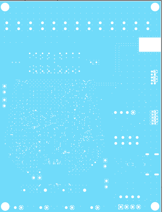
GND 3 (Scale 1:1)
